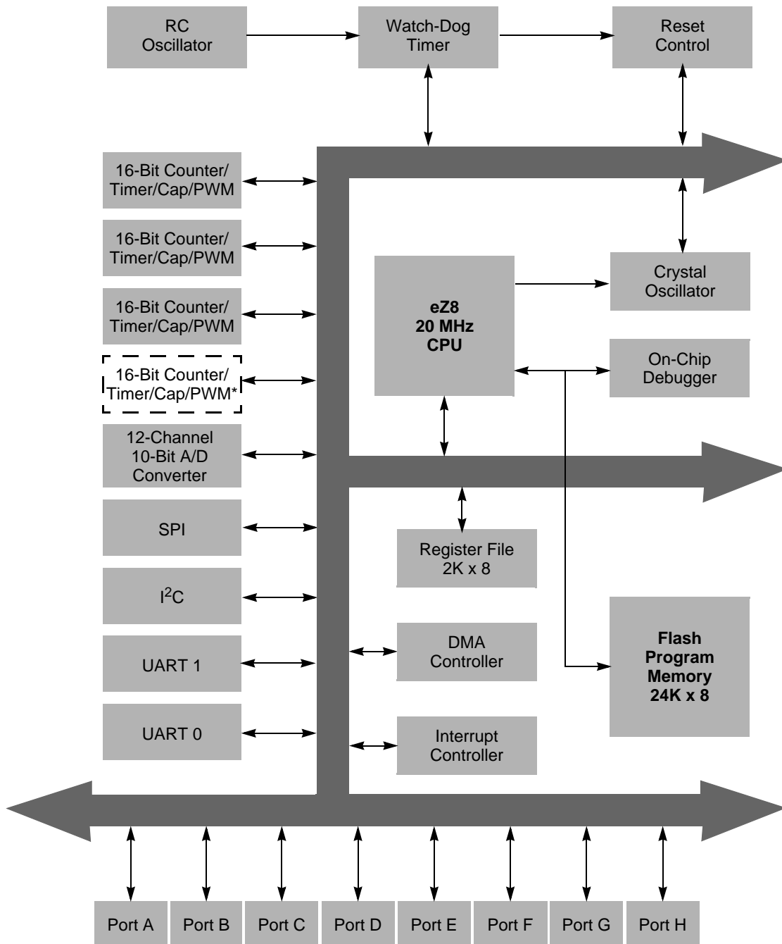
Figure 1. Z8F240x Block Diagram
