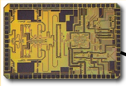
60GHz Integrated TX with PLL
