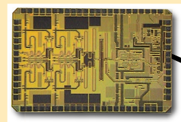
60GHz Integrated RX with PLL
