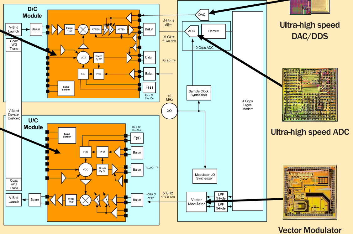
Millimeter-wave Datalink Example
