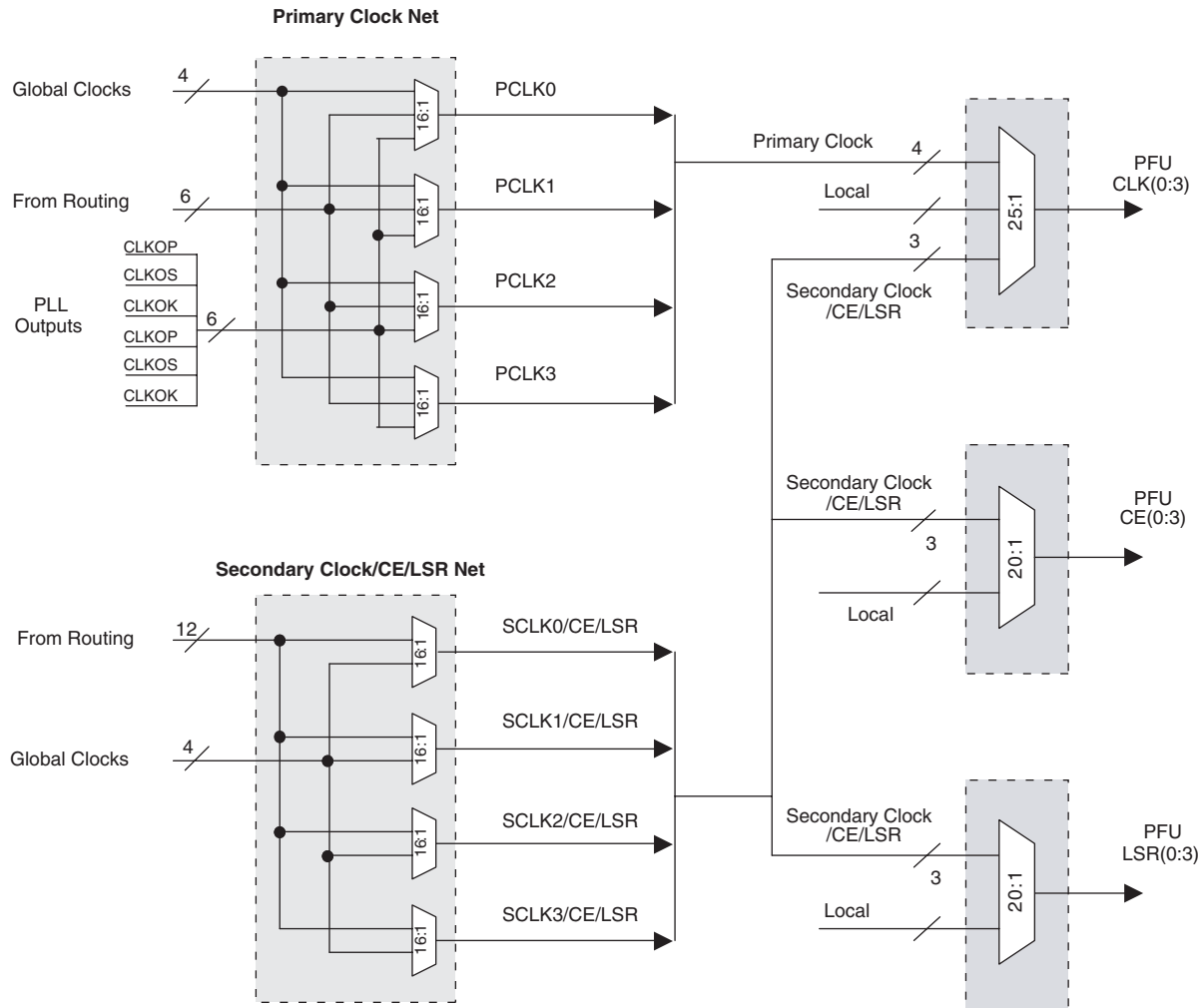
Figure 10-16. Primary Clock and Secondary Clock/CE/LSR Distribution
