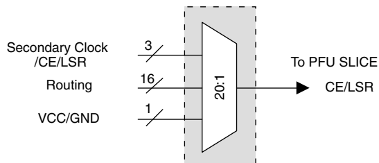
Figure 10-15. Control Switch Mux to Each PFU Slice
