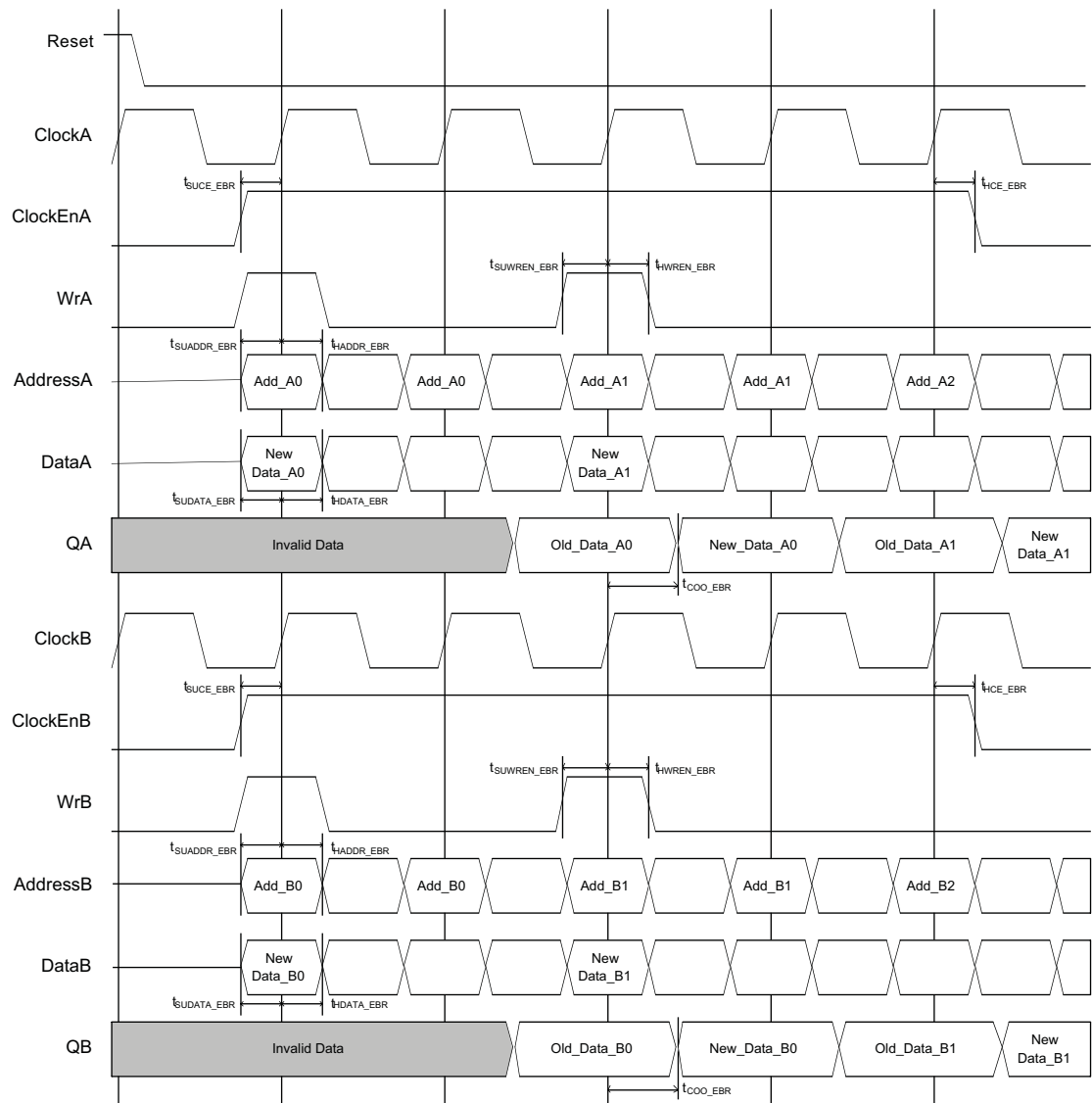
Figure 9-16. True Dual Port RAM Timing Waveform - READ BEFORE WRITE Mode, with Output Registers
