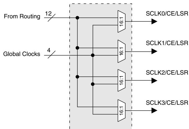
Figure 10-13. Secondary Clock/Control Net (All MachXO)
