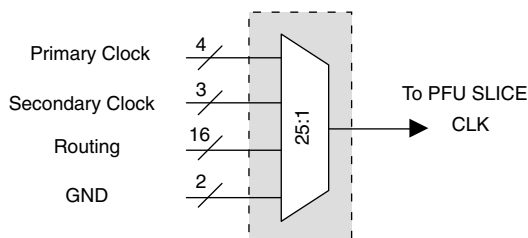
Figure 10-15. Control Switch Mux to Each PFU Slice
