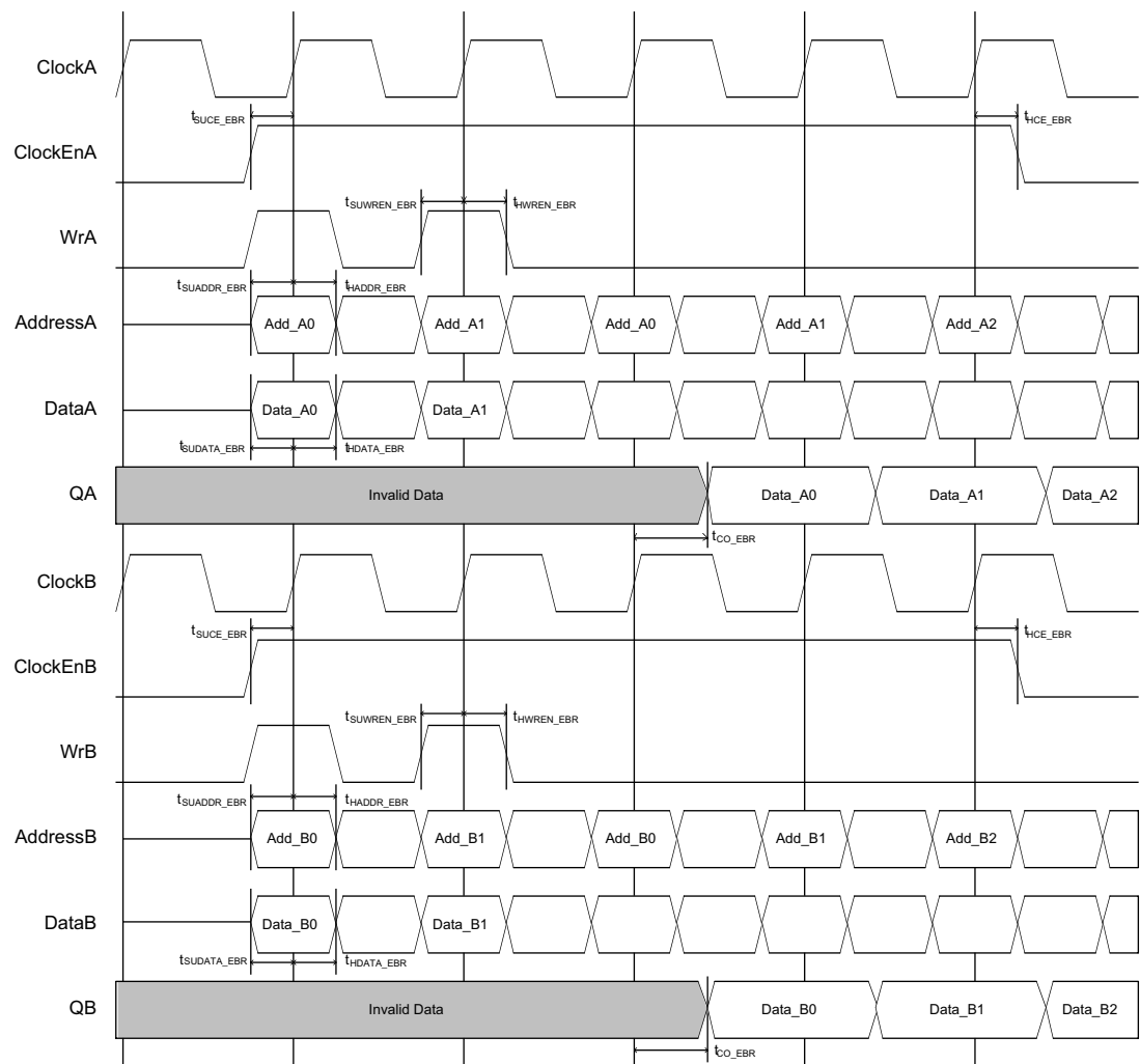
Figure 9-13. True Dual Port RAM Timing Waveform - NORMAL Mode, without Output Registers
