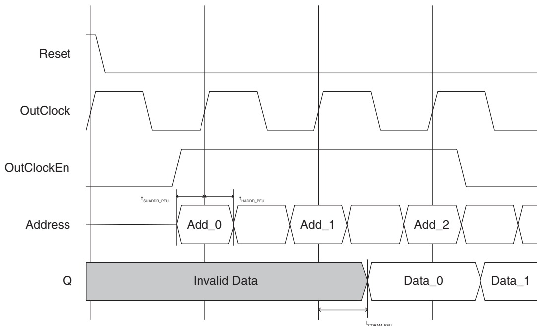
Figure 9-36. PFU-Based ROM Timing Waveform – with Output Registers
