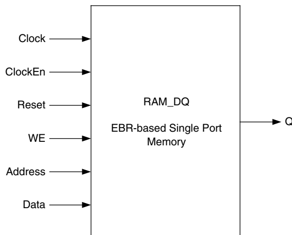
Figure 9-5. Single Port Memory Module Generated by IPexpress
