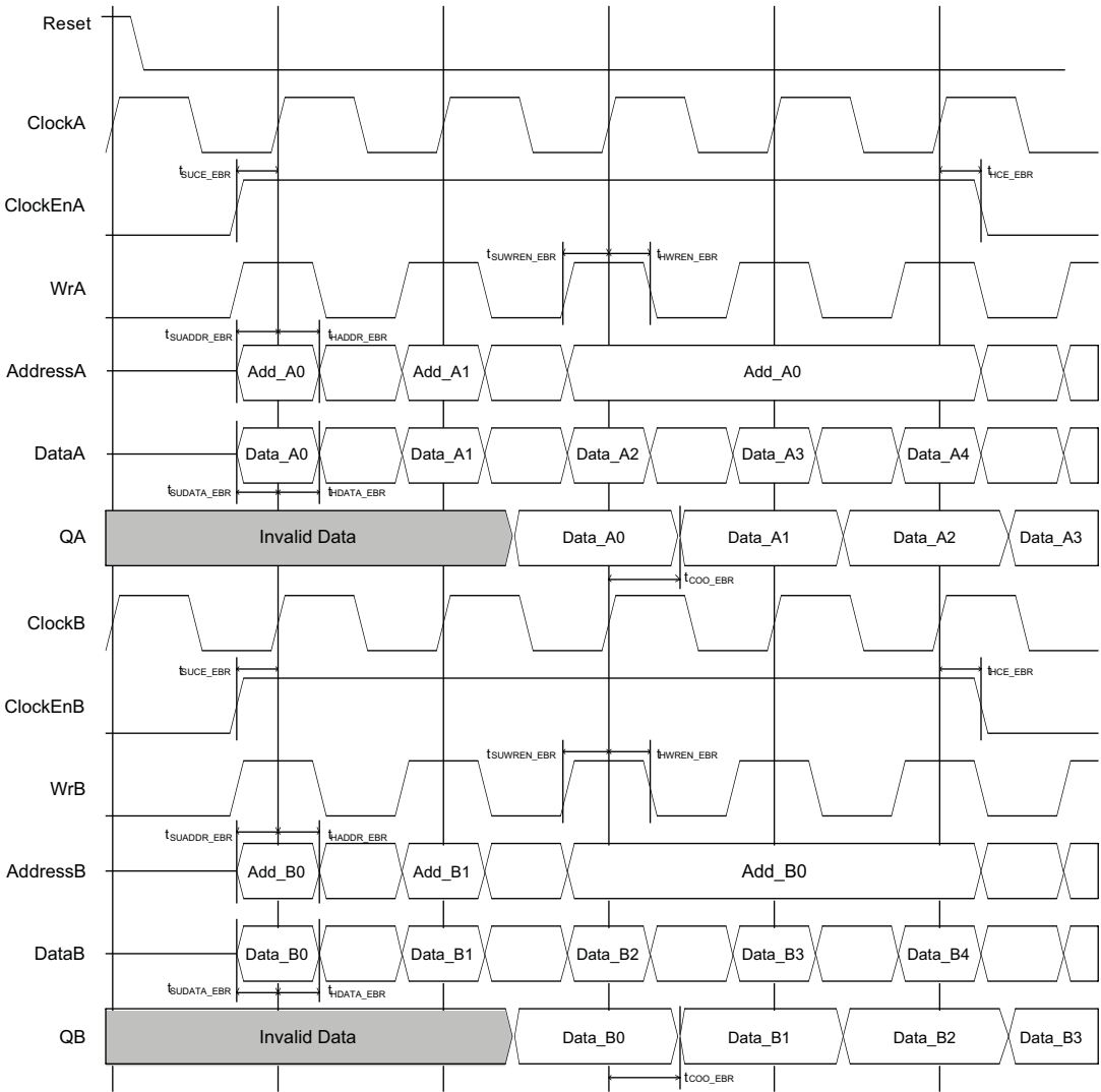
Figure 9-18. True Dual Port RAM Timing Waveform - WRITE THROUGH Mode, with Output Registers
