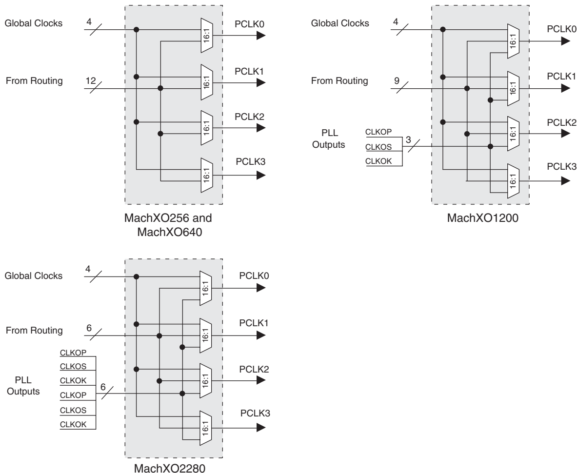
Figure 10-12. Primary Clock Net
